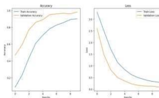
Figure. 4 CNN Accuracy and Loss
