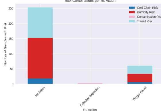
Risk Combinations per RL Action
