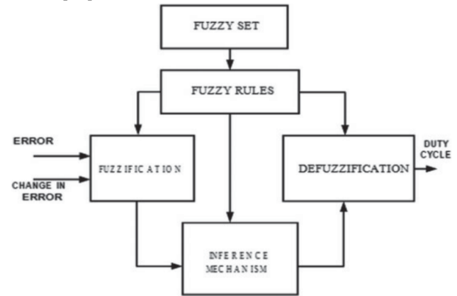
Figure.5 Fundamental FLC controller low
