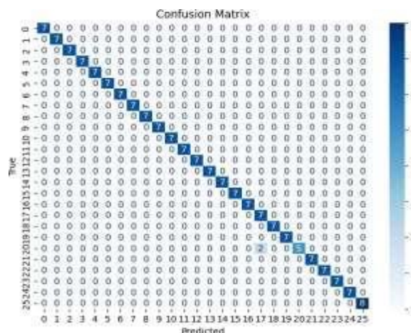
Figure. 6 Confusion Matrix for MobileNet
