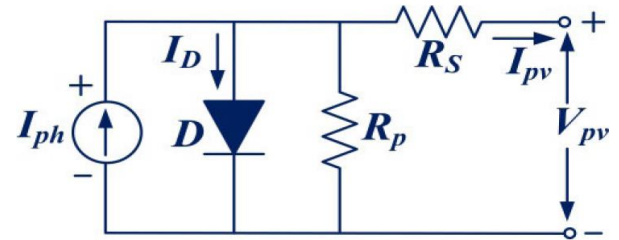
Figure.2 Equivalent circuit of solar cell
