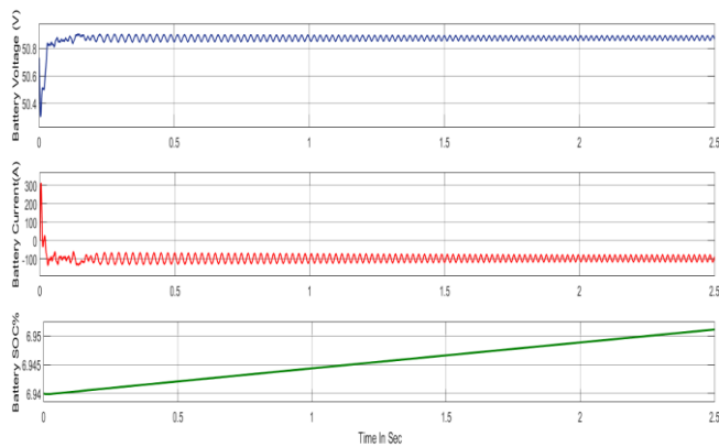
Figure. 9 Battery Charging Process when both sources are active
